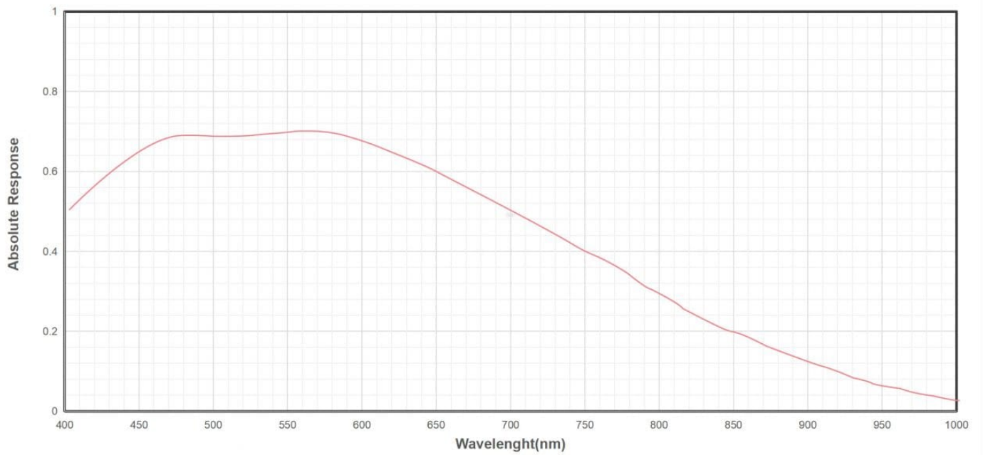
QHY1253 QE
